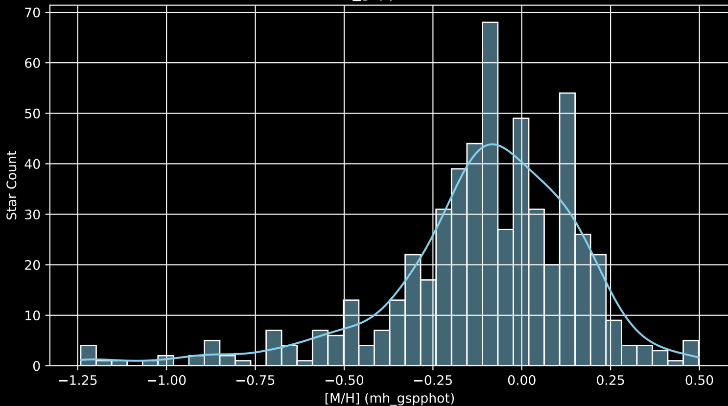
APOGEE DR17 Field: [120+08 [M/H] (mh_gspphot) (n= 557)
