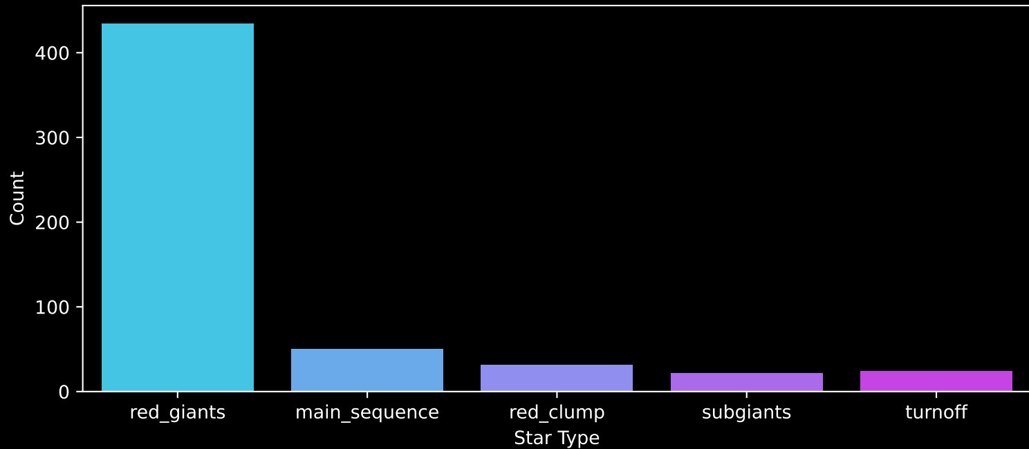
APOGEE DR17 Field: [120+08] Count plot of Star Type
