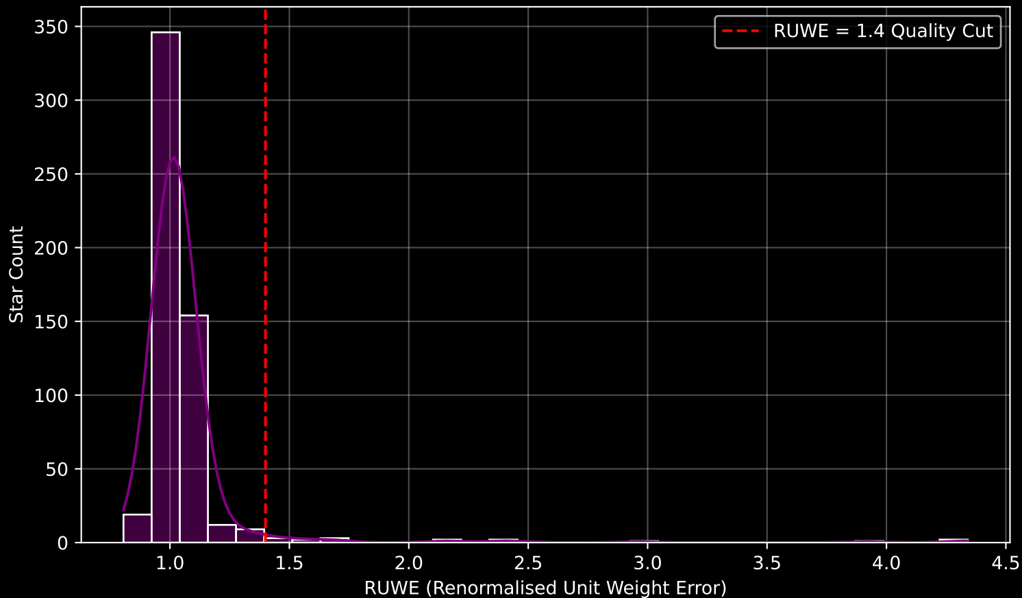
GAPOGEE DR17 Field [120+08] RUWE Distribution (n= 556)
