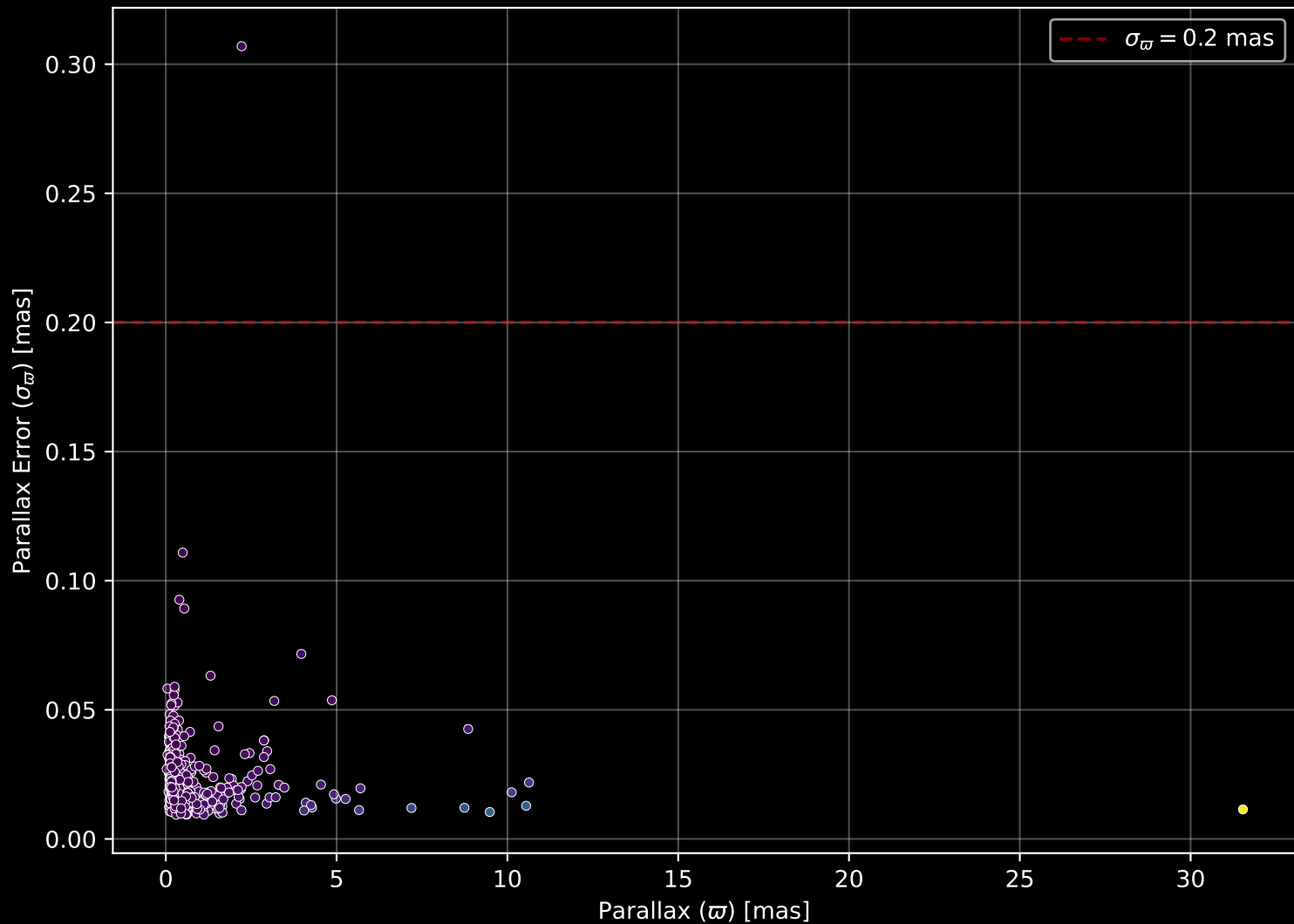
APOGEE DR17 Field: [120+08] Parallax Quality (n= 561)
