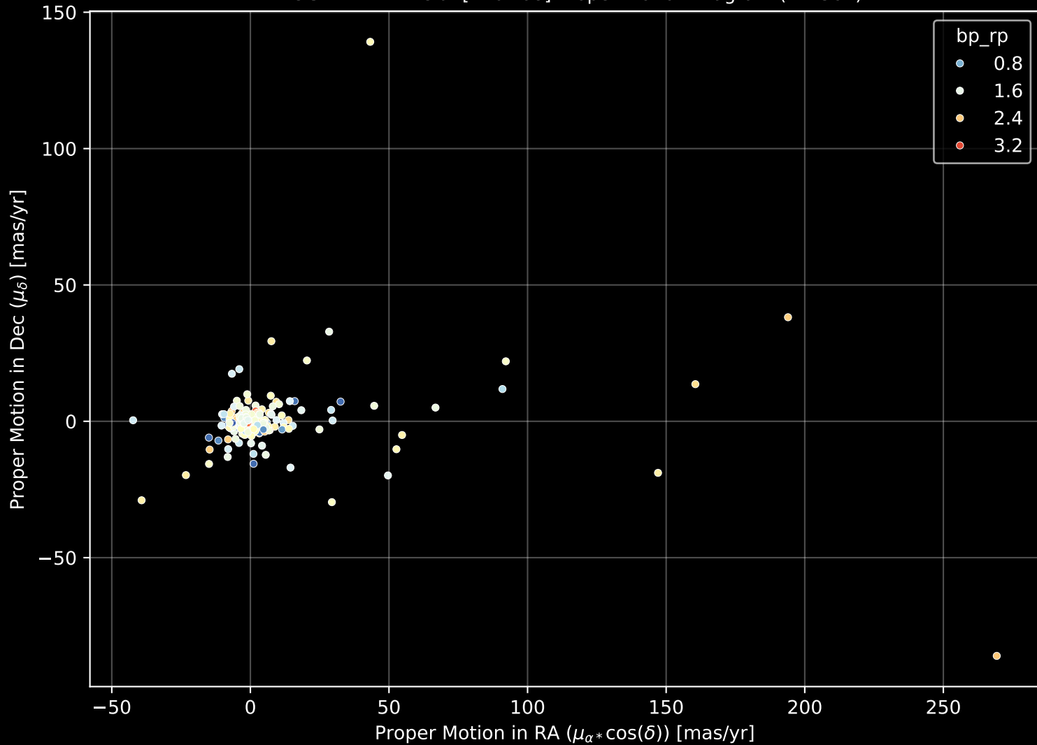
APOGEE DR17 Field: [120+08] Proper Motion Diagram (n= 561)
