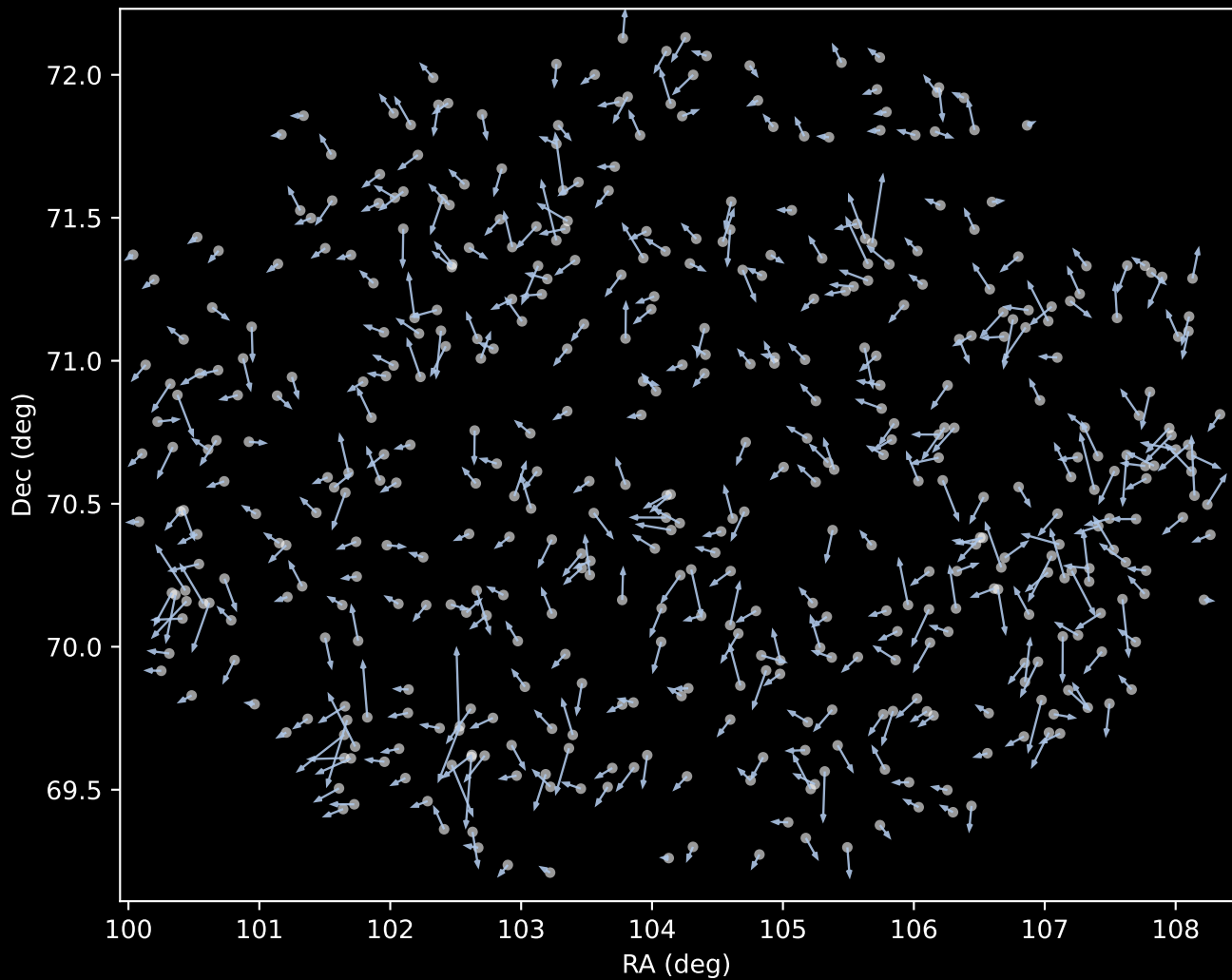
APOGEE DR17 Cluster 1 Proper Motion Vectors (n=462)
